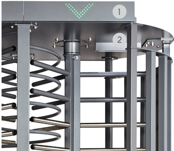
Indicative LEDs available as an optional item (1) and internal lighting (2). Arms in stainless steel at the point where users touch the equipment.
